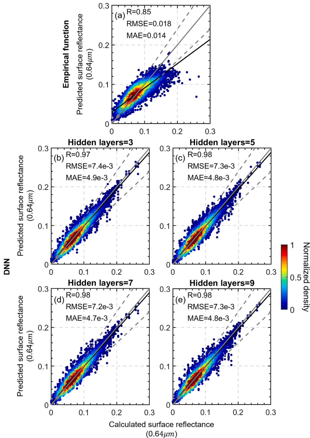
Fig. 4. (a) Density scatterplots of the comparison between surface reflectance ( SR ) at 0.64 \mu m ( SR_{0.64} ) predicted by the empirical function and SR_{0.64} calculated from Eqs. 1–3, the “true” surface reflectance. (b–e) Density scatterplots of 10-cross-validation results for SR_{0.64} derived from DNN, considering different numbers of hidden layers in the DNN model. The correlation coefficients ( R ), root-mean-square errors ( RMSE ), and mean absolute errors ( MAE ) are given in each panel. The solid black lines represent the best-fit lines from linear regression. The dashed grey lines are plotted as Y = 0.8 \times and Y = 1.2 \times (positions of 20% error).
