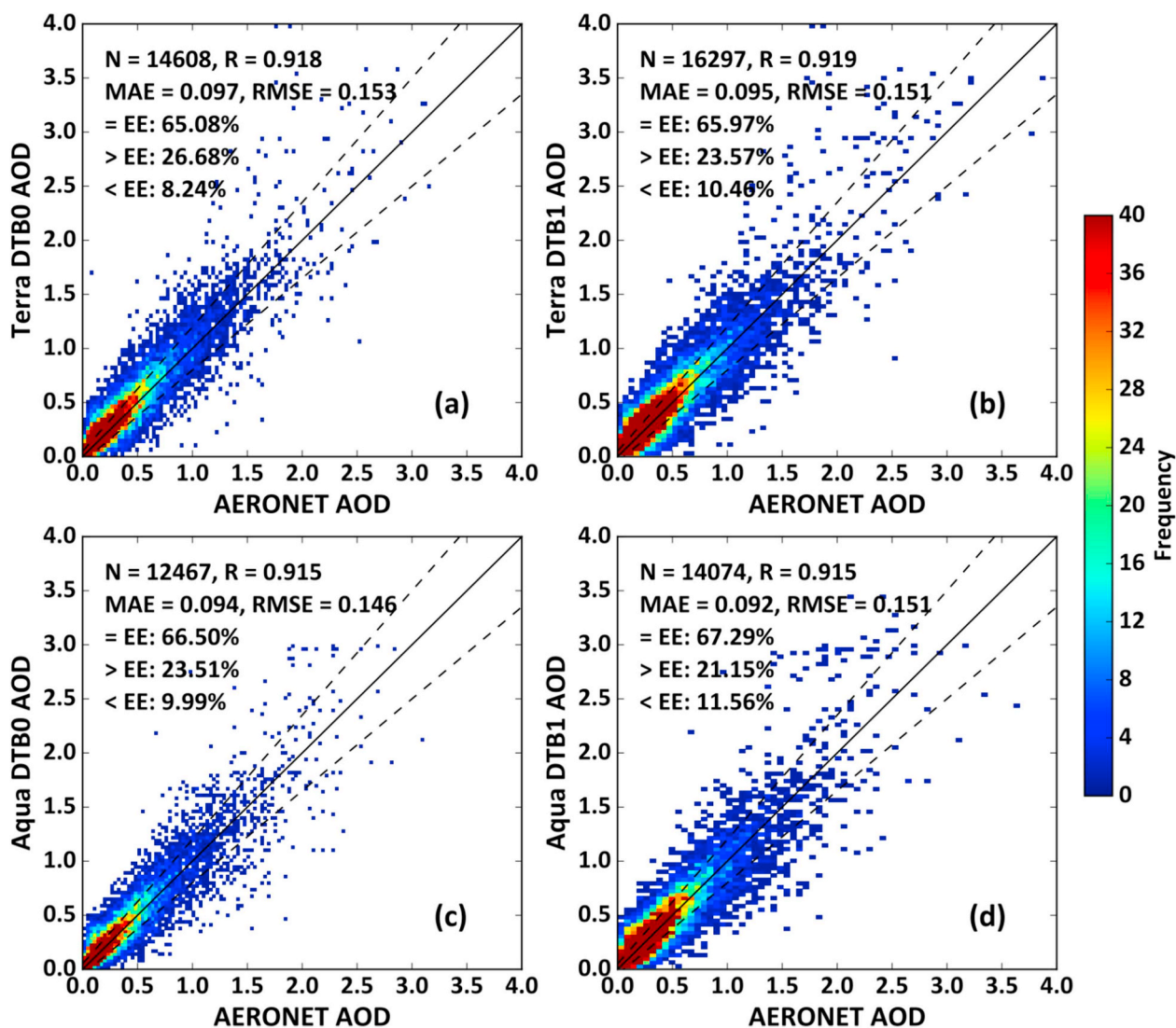
Fig. 7. Same as Fig. 5 but for Asia.
