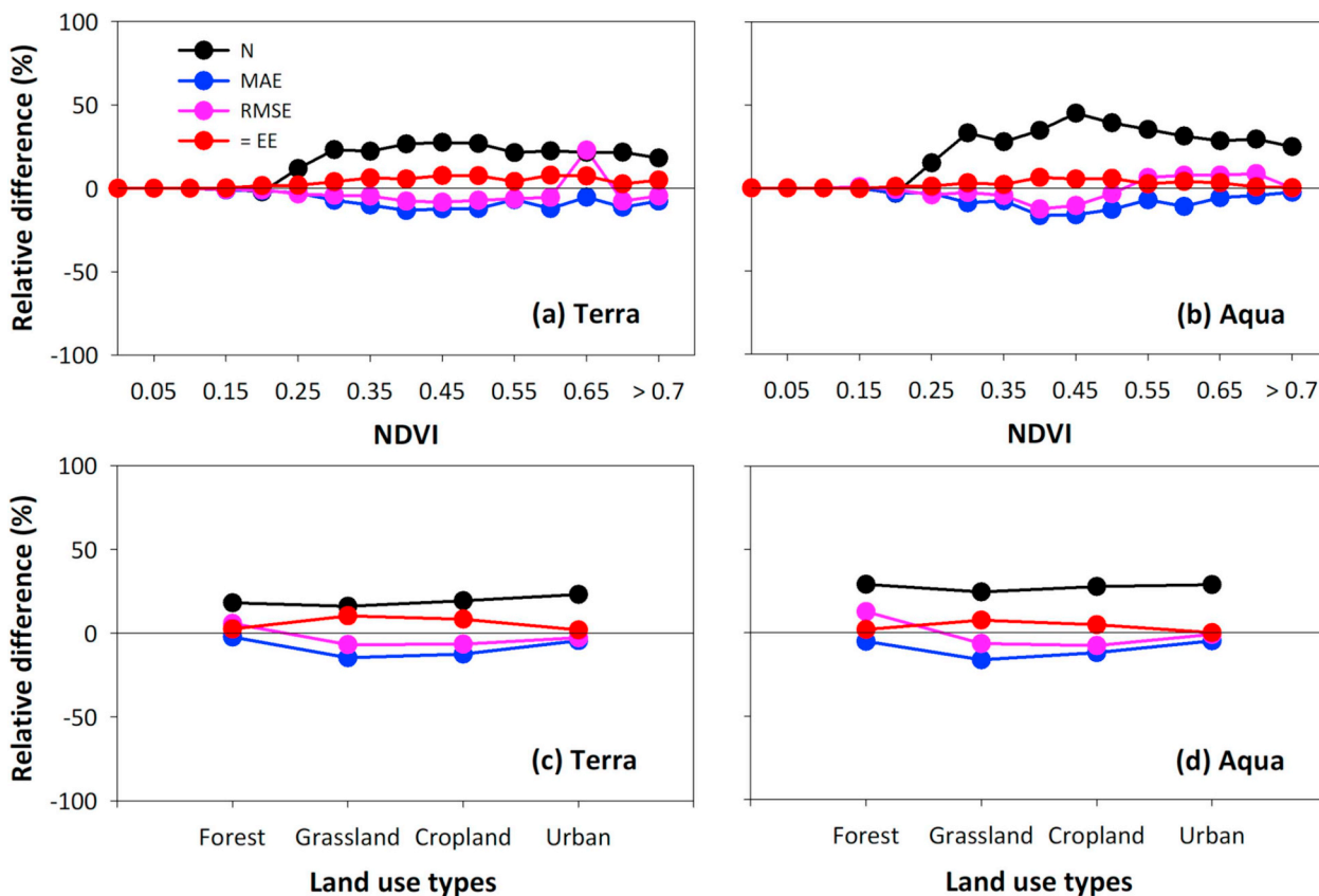
Fig. 10. Relative differences (%) between DTB0 and DTB1 AOD products against AERONET AOD retrievals as a function of (a, b) NDVI and (c, d) land use type for Terra (left panels) and Aqua (right panels) over land.
