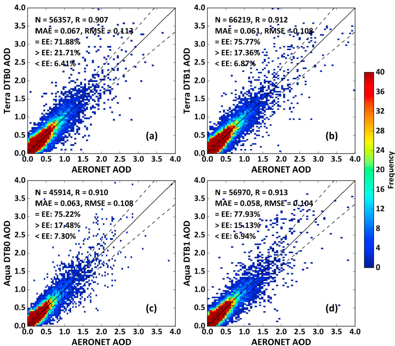
Fig. 9. Same as Fig. 5 but for the globe.
