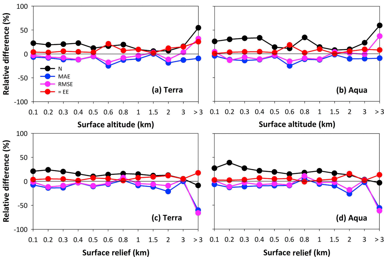
Fig. 11. Same as Fig. 10 but for (a, b) surface altitude and (c, d) surface relief.
