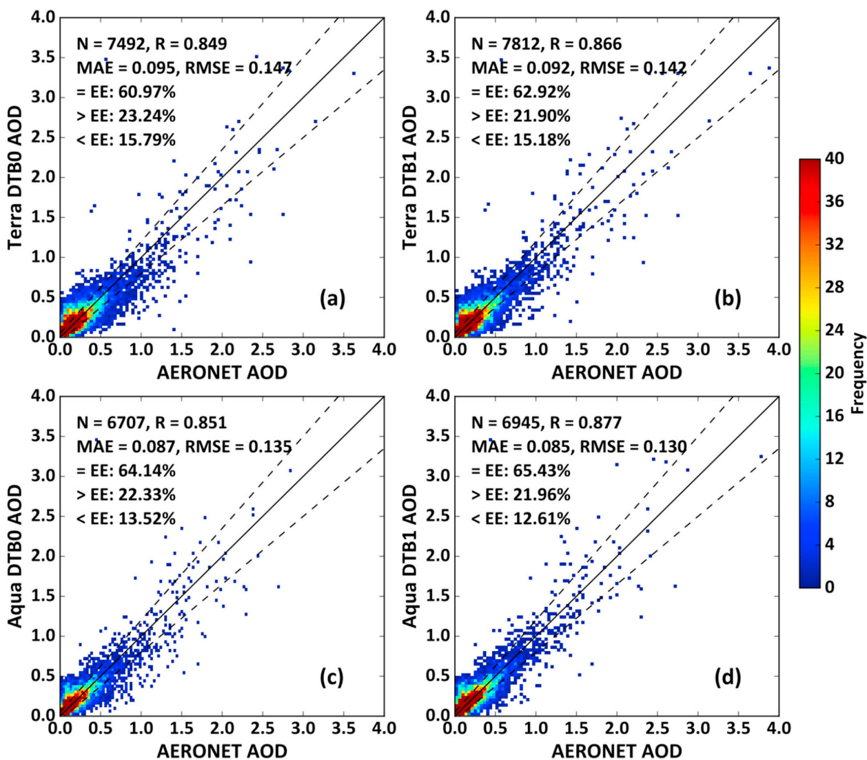
Fig. 8. Same as Fig. 5 but for Africa.
