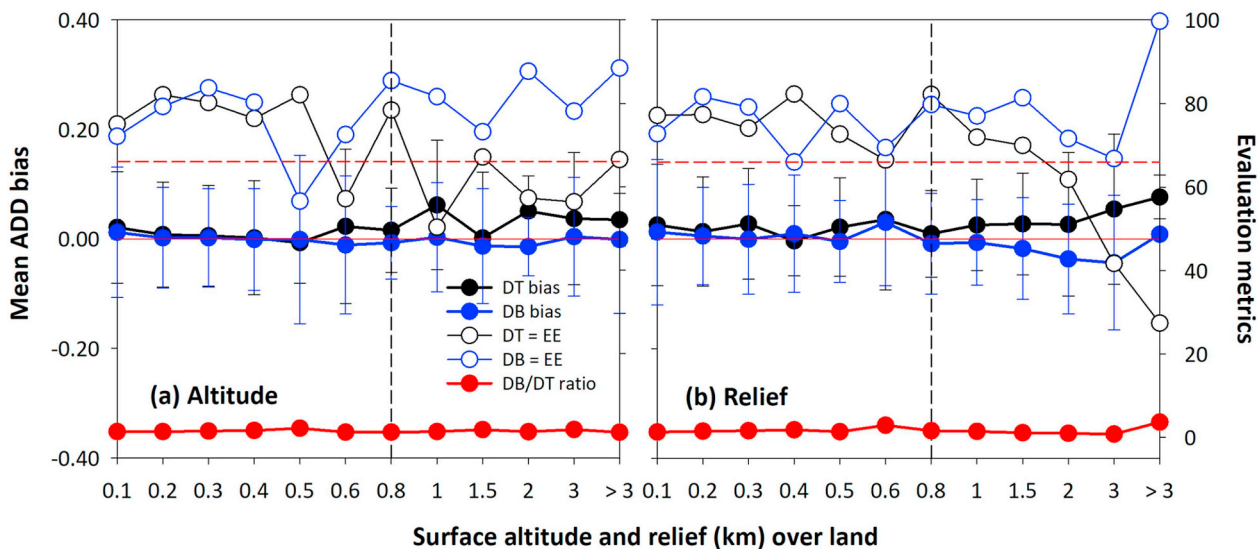
Fig. 3. Same as Fig. 2 but for (a) surface altitude and (b) surface relief.
