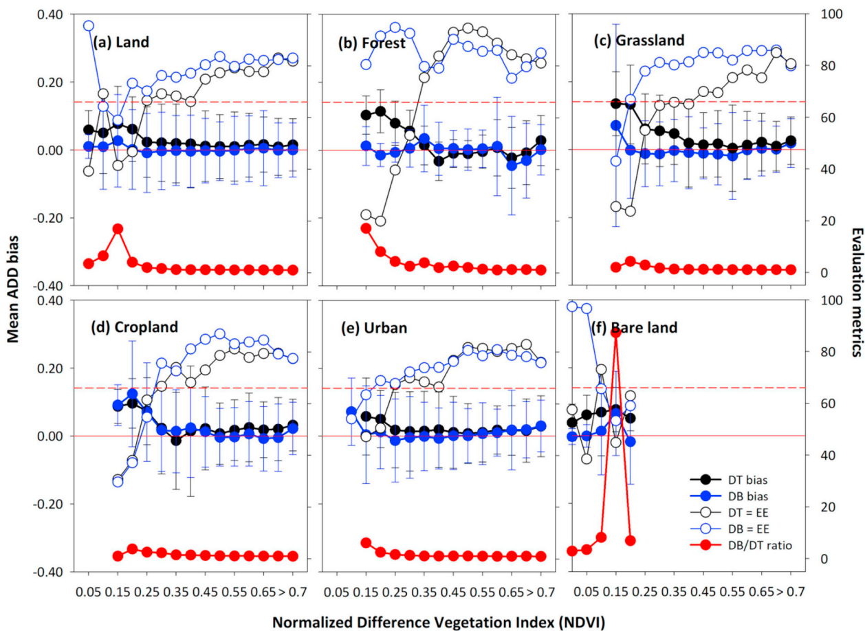
Fig. 2. Mean aerosol optical depth (AOD) bias (black, filled circles for the DT algorithm and blue, filled circles for the DB algorithm), fraction of retrievals matching the expected error (EE, black, open circles for the DT algorithm and blue, open circles for the DB algorithm), and the data-count (DB/DT) ratio (red, filled circles) as a function of NDVI for six land use types. The bias is calculated with respect to AERONET AOD retrievals. The red horizontal solid and dotted lines represent the zero bias ( X = 0 ) and “good” matching lines. (For interpretation of the references to color in this figure legend, the reader is referred to the Web version of this article.)
