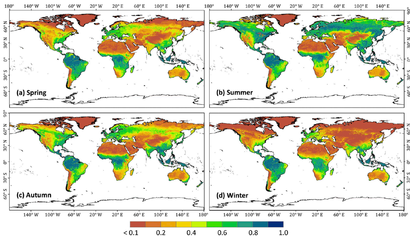
Fig. 1. Seasonally averaged normalized difference vegetation index maps from 2013 to 2017 over land.
