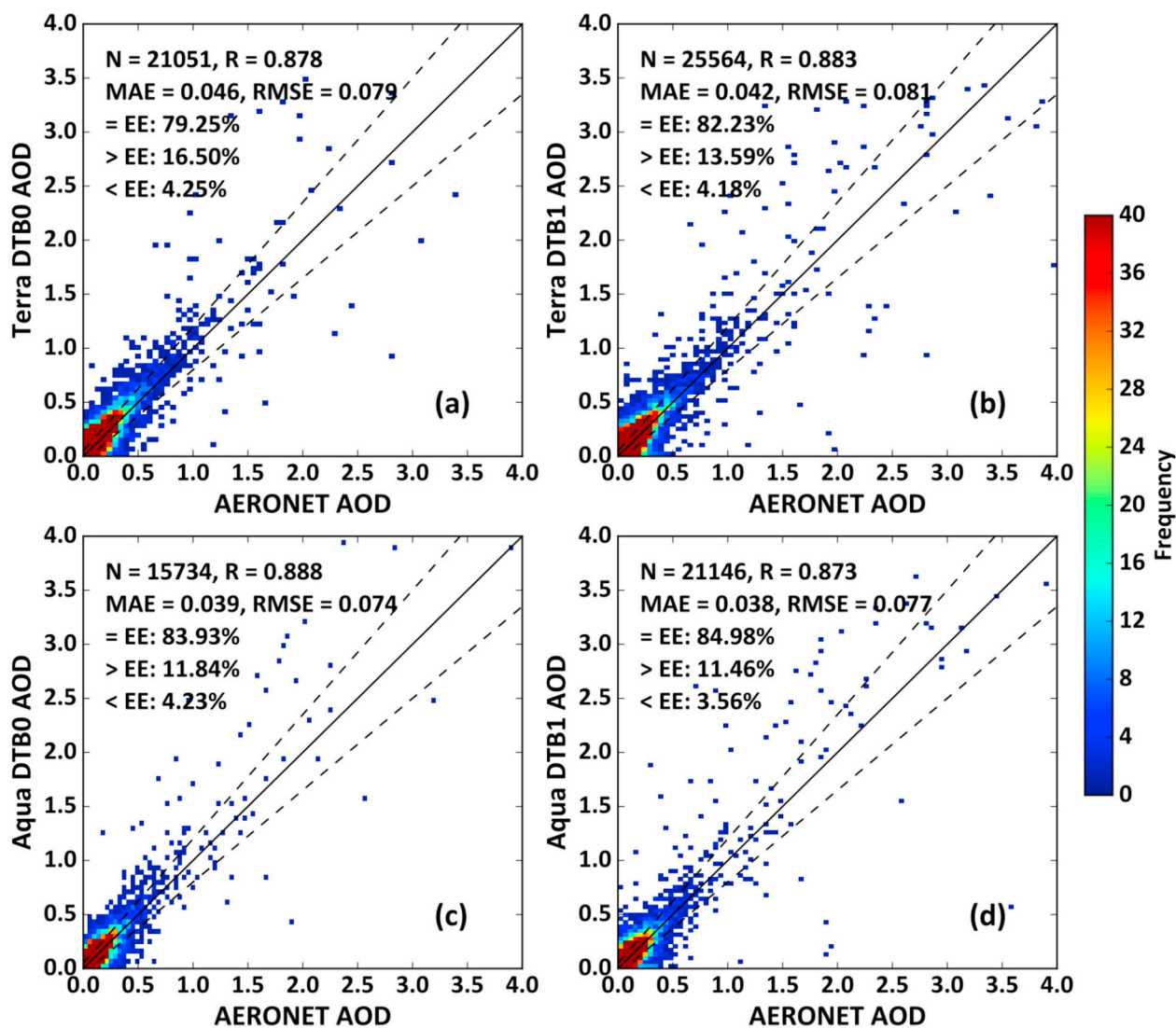
Fig. 6. Same as Fig. 5 but for North and South America.
