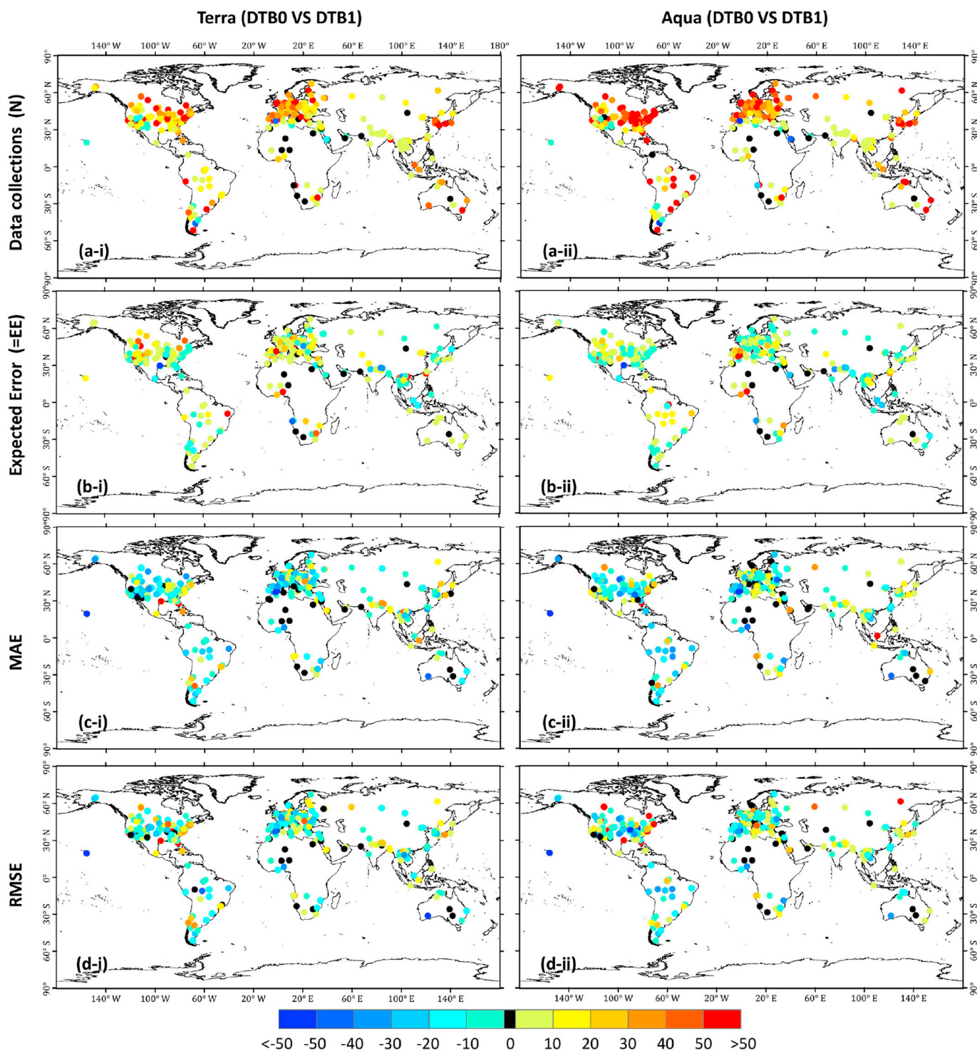
Fig. 4. Spatial distributions of the better performing product for Terra (i) and Aqua (ii) combined DT and DB products based on the evaluation metrics: (a) number of data samples (N), (b) percentage of data within the EE envelope, (c) MAE, and (d) RMSE.
