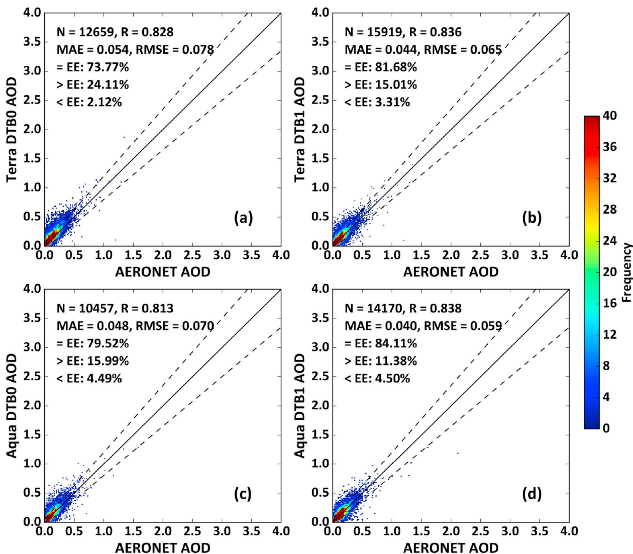
Fig. 5. Density scatter plots of Terra and Aqua MODIS C6.1 DTB0 and DTB1 AODs as a function of AERONET AOD measurements over Europe from 2013 to 2017. The black solid line is the 1:1 line, and the dashed lines outline the EE envelope.
