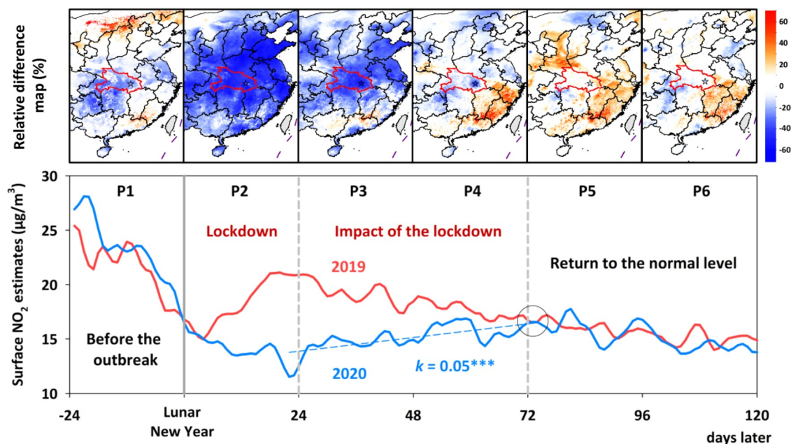
Figure 5. Time series of the 3-day moving average of daily surface NO 2 concentrations ( \mu\text{g}/\text{m}^3 ) in China (bottom panel) and the relative difference (%) in surface NO 2 concentrations ( \mu\text{g}/\text{m}^3 ) between 2020 and 2019 (top panel) during six periods (i.e., P1–P6) in eastern China before and after the Lunar New Year. The red border and star in the top panel indicate Hubei Province and Wuhan City, respectively. The gray circle in the bottom panel highlights when the surface-measured NO 2 concentration from 2020 reached the 2019 historical level. The dashed blue line shows the linear trend for observations during the period experiencing the impact of the lockdown in 2020. The slope ( k ) is given, and the three asterisks indicate p < 0.001 .
